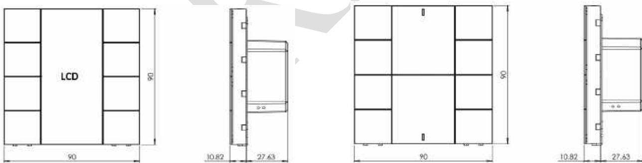
Fig 3 : Dimensions of the iSwitch
