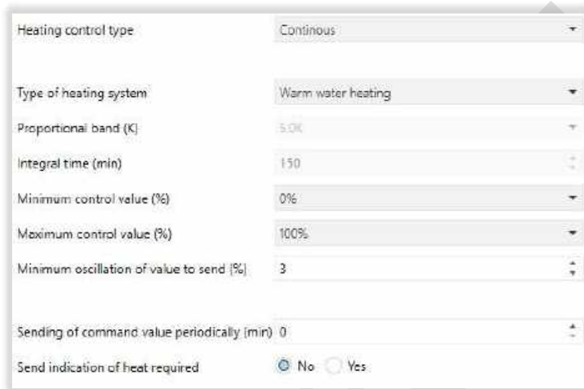
Fig 26 : Heating Continuous Control Configuration
