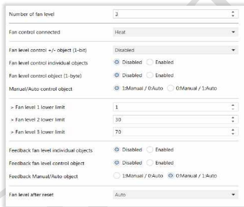
Fig 35 : Fan Control Configuration Used For Room Controller
