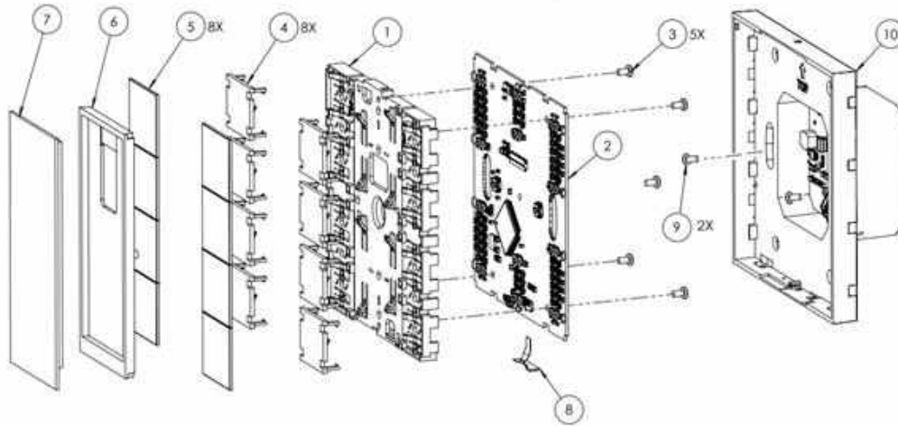
Fig 7 : Internal Componenets of Models with LCD
