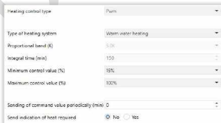
Fig 25 : Heating PWM Control Configuration
